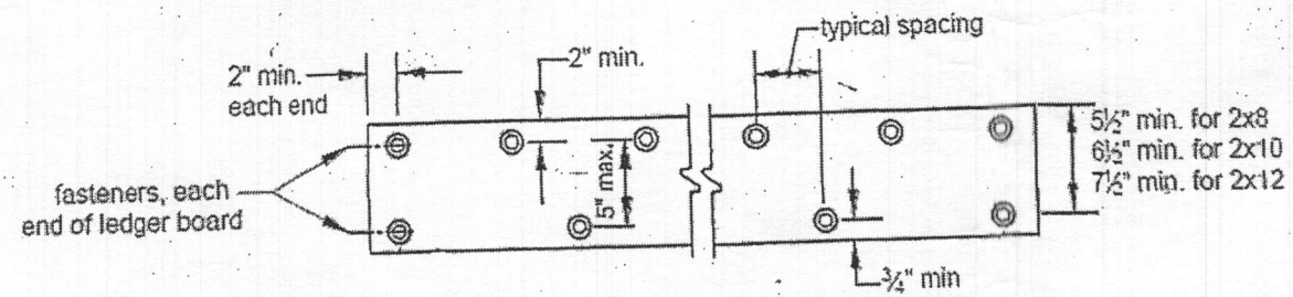
LEDGER BOARD FASTENER SPACING AND CLEARANCES
