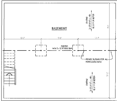
BASEMENT PLAN
