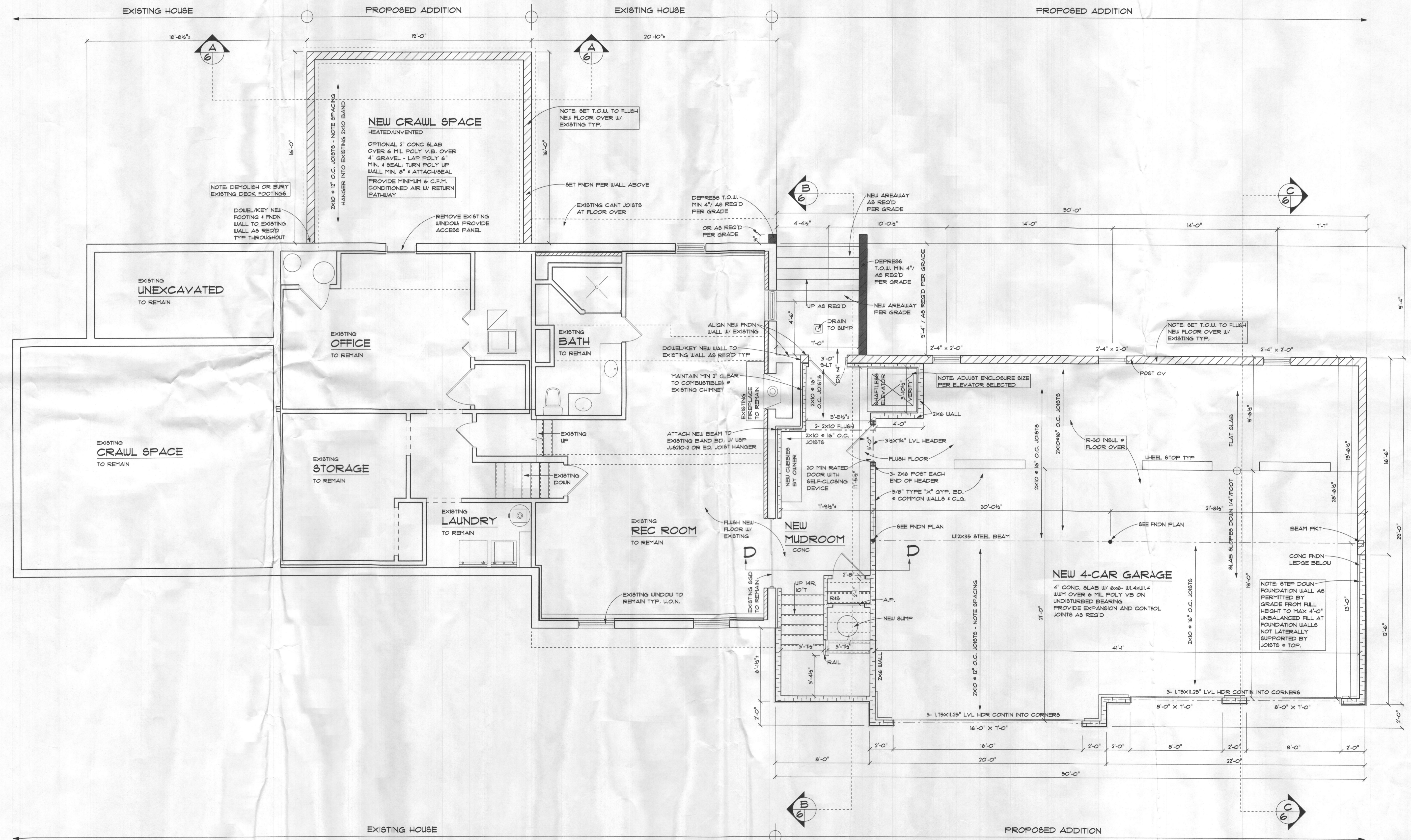
Proposed Lower Level Plan SCALE: 1/4" = 1'-0"
