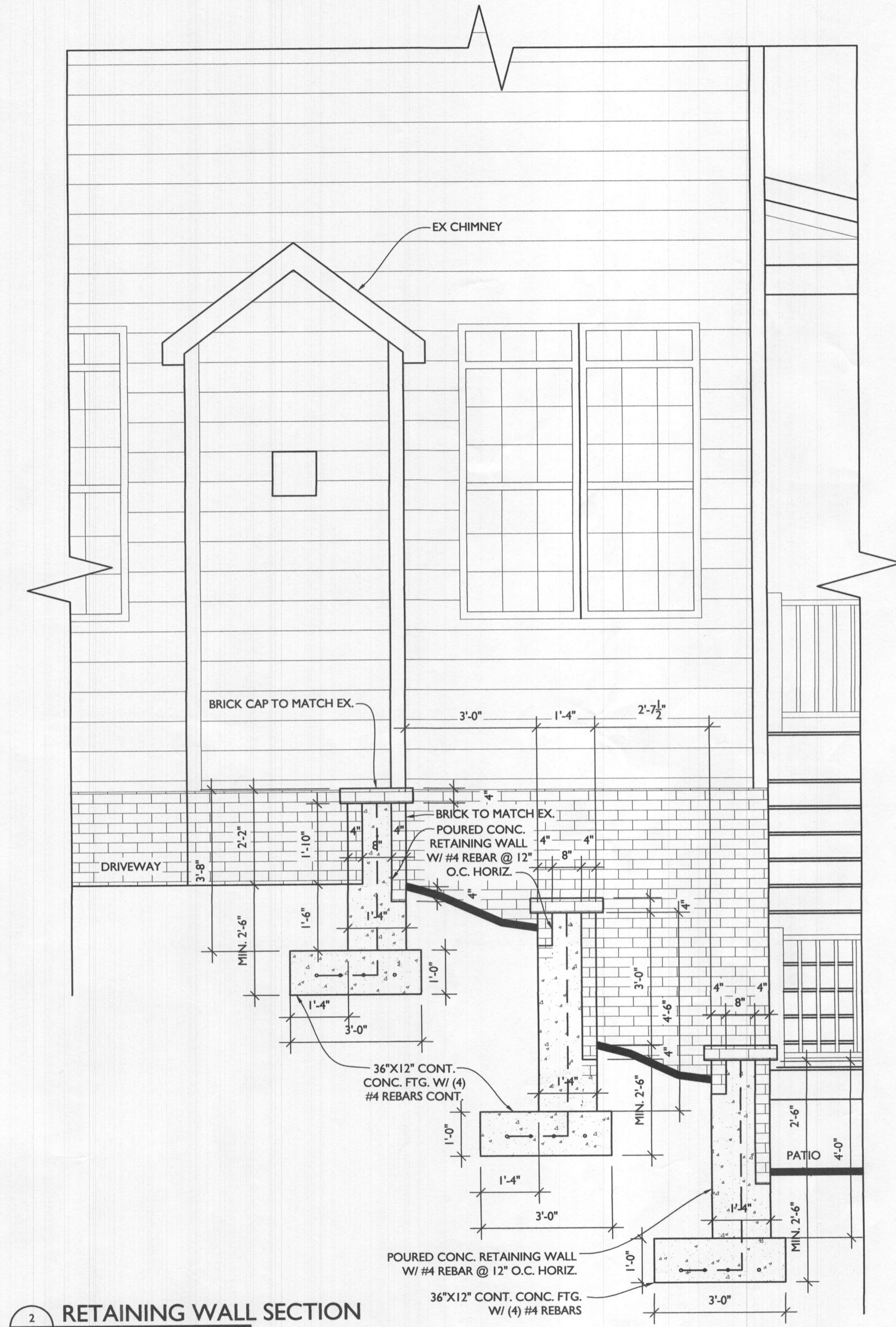
2 RETAINING WALL SECTION A301 SCALE: 1/2"=1'-0"
