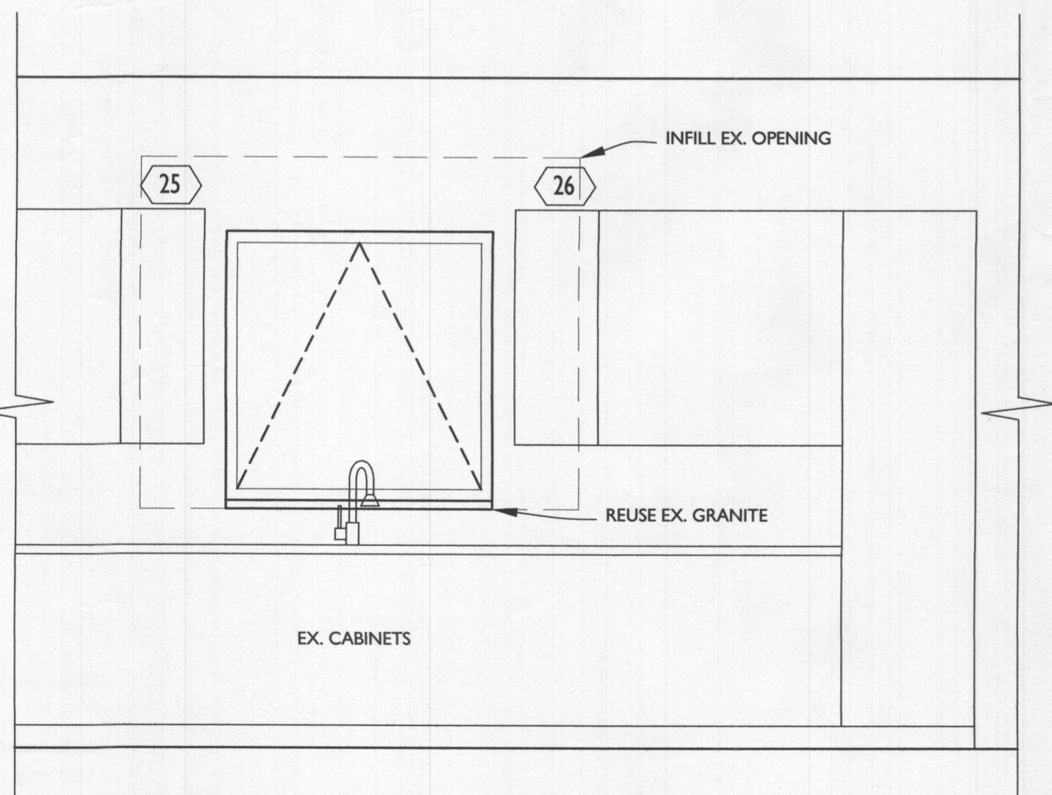
2 KITCHEN ELEVATION A201 SCALE: 1/2"=1'-0"
