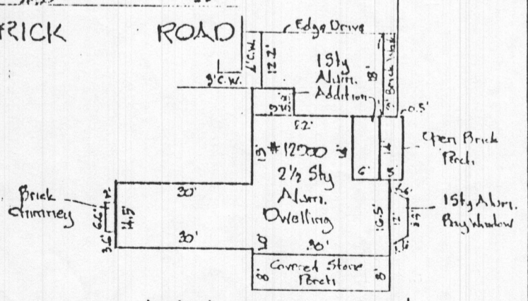
ENLARGED VIEW 1" = 30'
