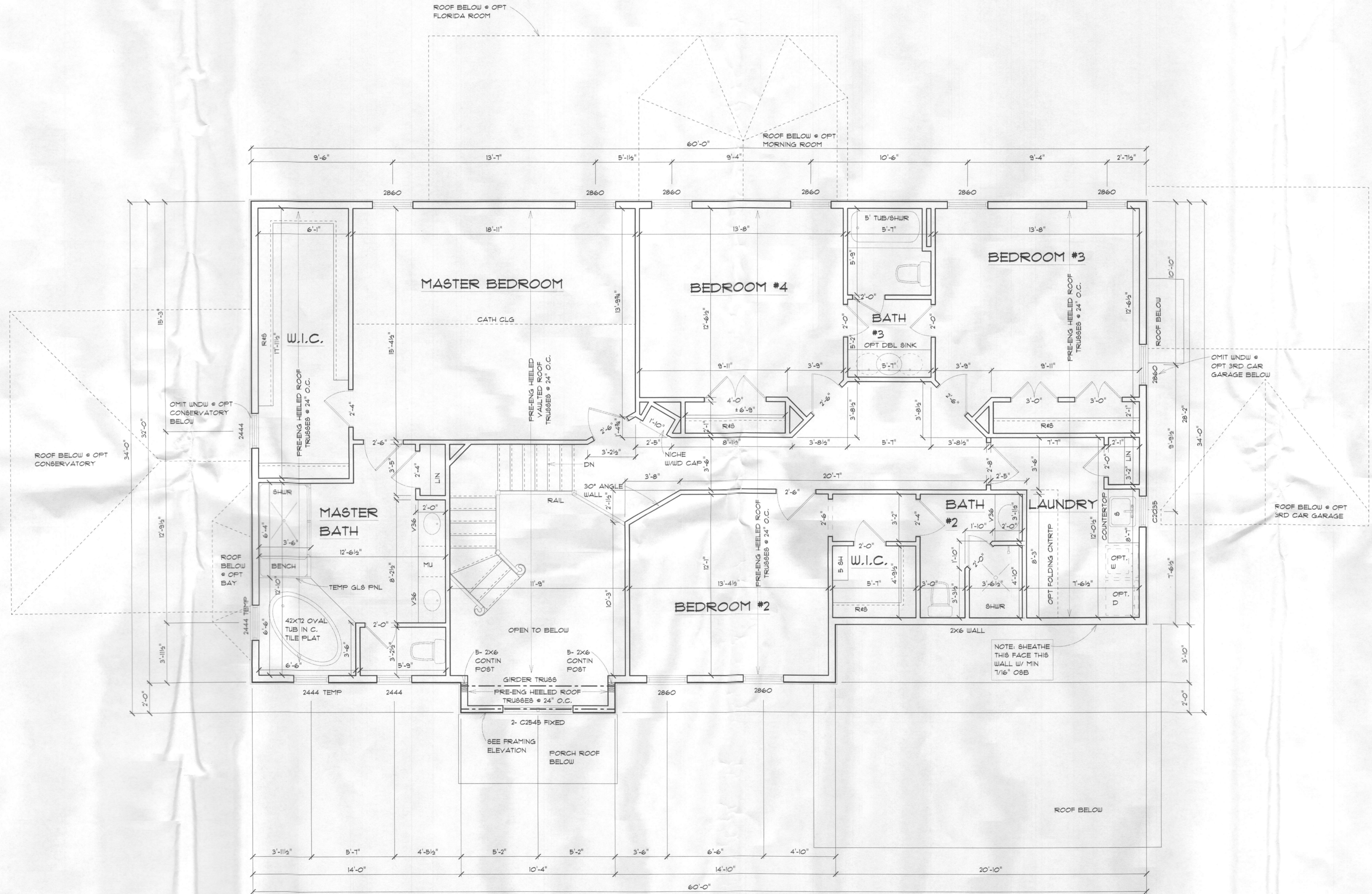
SECOND FLOOR PLAN @ ELEVATION A - STANDARD
