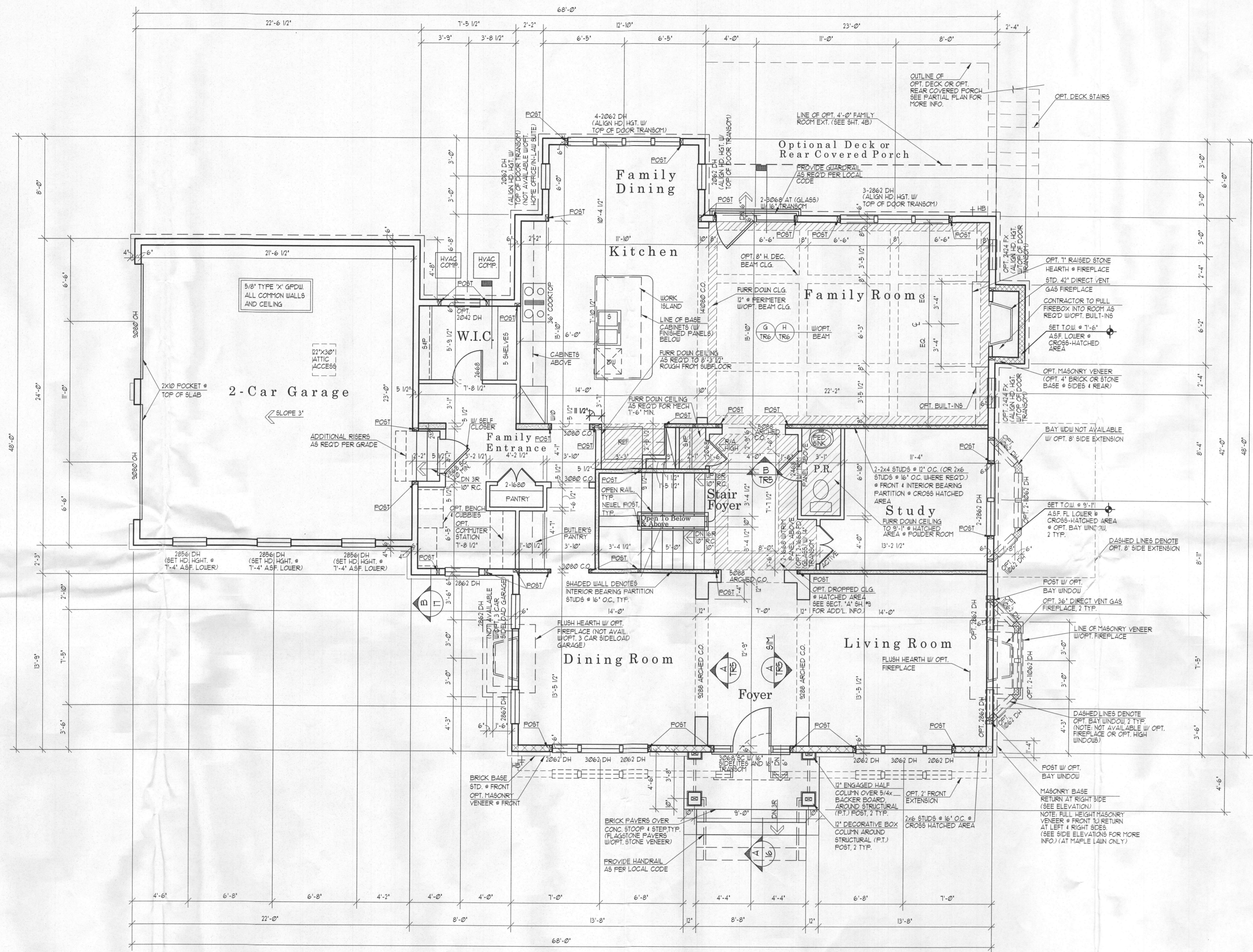
LOWER FLOOR PLAN W/ELEVATION "A" 1/4" = 1'-0" UNLESS OTHERWISE NOTED ALL INTERIOR PARTITIONS TO BE 3/4" UNLESS OTHERWISE NOTED WINDOW HEAD HEIGHT TO BE 8'-0" A.S.F. UNLESS OTHERWISE NOTED PROVIDE 2x2x6 POSTS BETWEEN ALL MULTIPLE WINDOWS.
