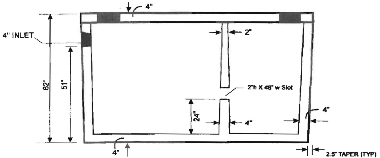
SECTION VIEW
