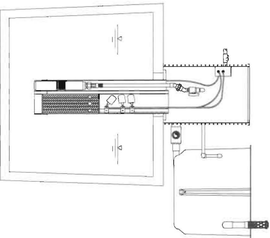
End View
